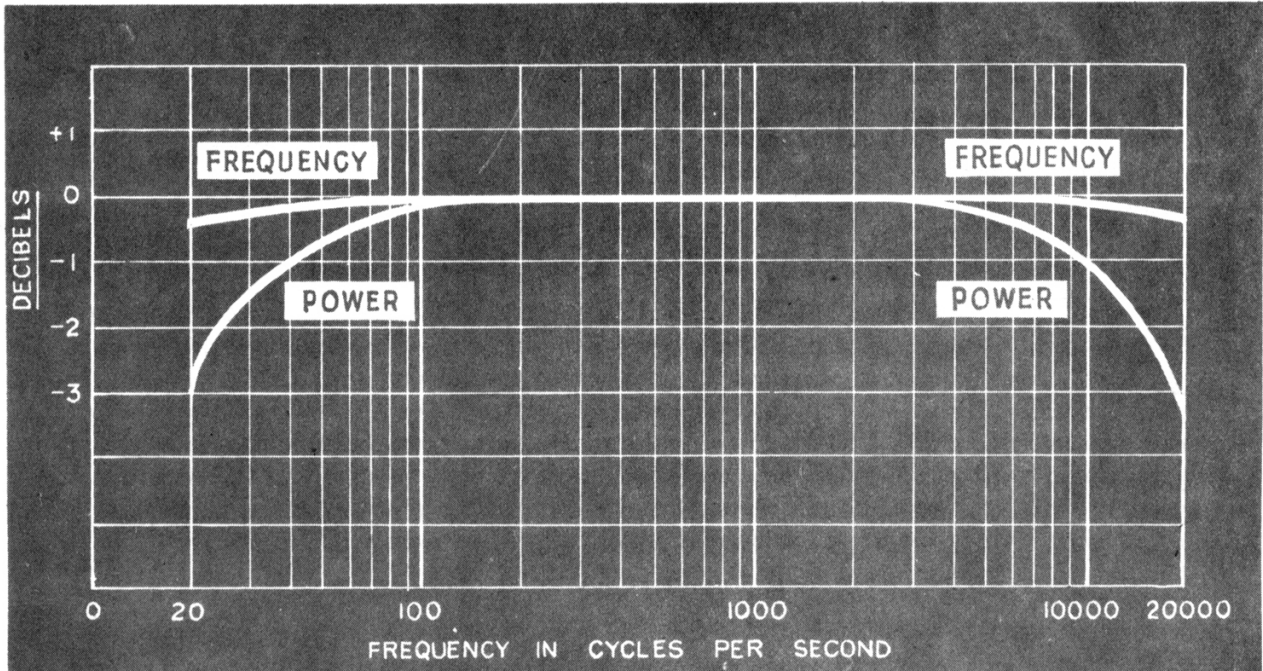
THIS CURVE REPRESENTS THE MAXIMUM EXPECTED POWER & FREQUENCY DEVIATION FROM THE RATED MID-RANGE VALUE
